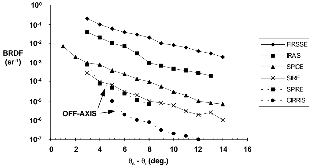
Figure 3-6. BRDF measurements for selected space sensors.
