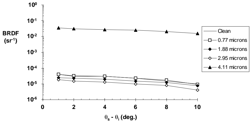
Figure 3-13. Effect of H 2 O deposition on 16K mirror BRDF - 10.6 μm.
